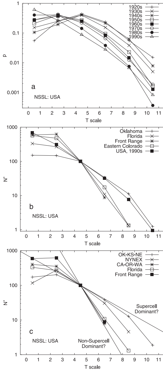
Fig. 2. USA tornado intensity distributions p(F) plotted over T scale: (a) decadal data from 1920 to 1999, (b) normalized regional distributions N^*(F) (1950–1999) compared to total USA in the 1990s, (c) categorization of regional N^*(F) distributions into likely supercell or non-supercell storm dominance. For N^*(F) in (b) and (c), the number of F2 tornadoes is fixed to 100.
