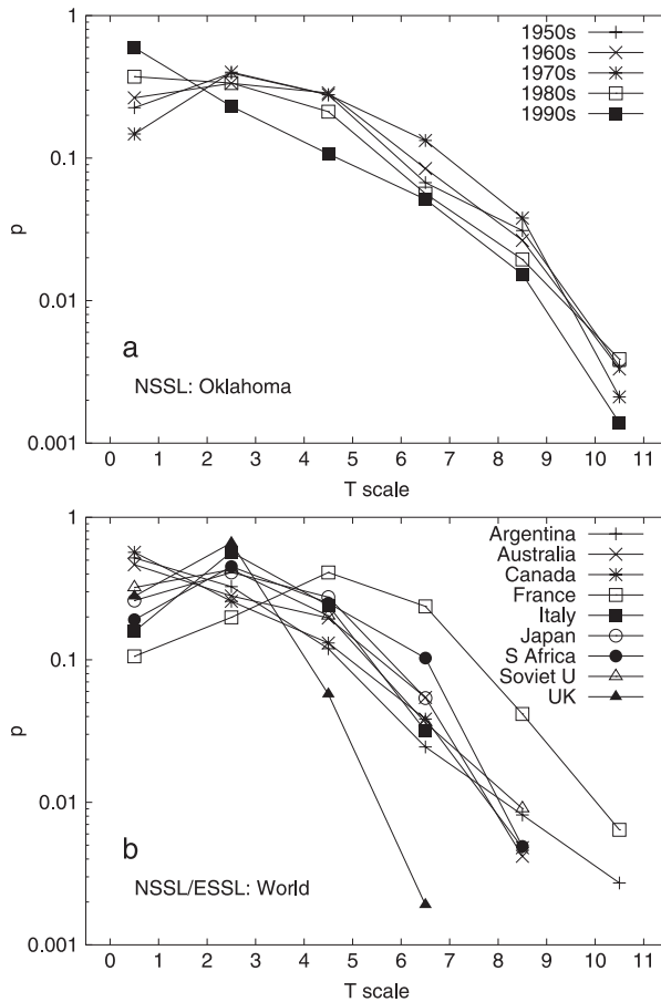
Fig. 3. Distributions p(F) plotted over T scale for (a) Oklahoma in the decades from 1950 to 1999 and (b) various countries all over the world.
