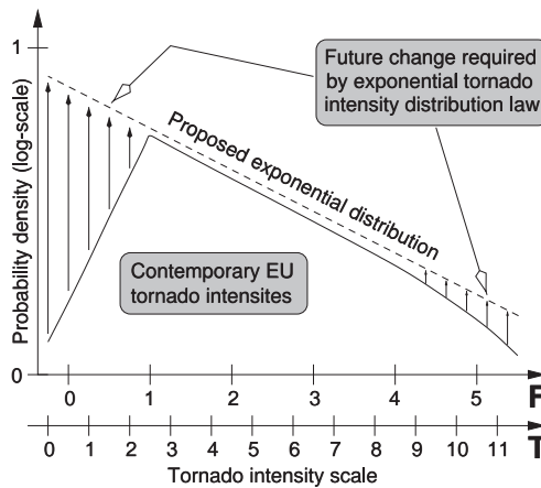
Fig. 1. Schematic diagram of most contemporary European tornado intensity distributions over T and F scales (solid, also valid for the USA before 1960) and required future changes (arrows) to an earlier-proposed climatological exponential distribution (dashed).
