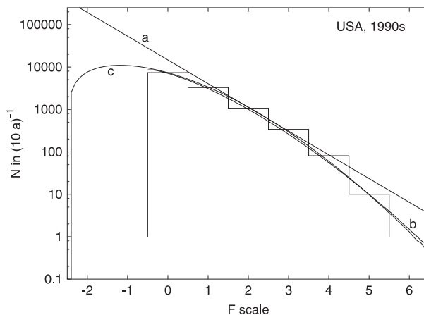
Fig. 5. Comparison of three different fits to the observed USA 1990s decadal intensity distribution with F scale (step function) according to Table 2: (a) exponential fit, (b) Weibull fit in v starting at F0 intensity ( 18 \text{ m s}^{-1} ) and (c) Weibull fit in v starting at F-2 intensity ( 0 \text{ m s}^{-1} ).
