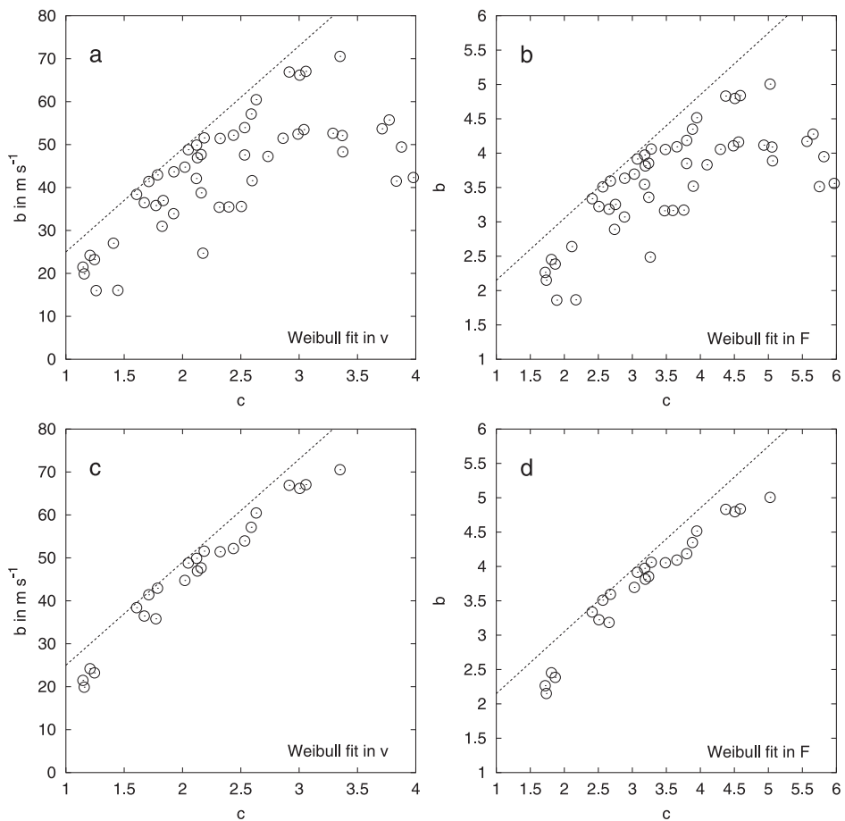
Fig. 6. Climatological cb -plots of Weibull parameters c and b for fits starting at F -2, i.e. v=0 \text{ m s}^{-1} : (a, c) fits in v ; (b, d) fits in F . Data from Tables 3 and 4. In panels (c) and (d), only data from regions with F5 tornadoes are depicted.
