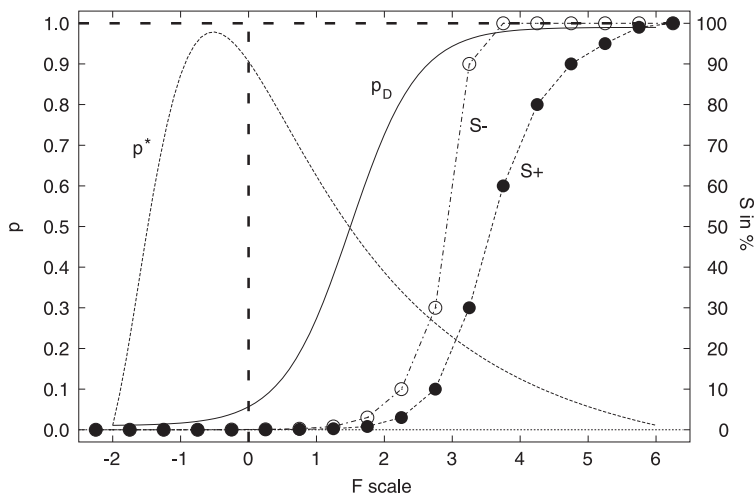
Fig. 7. Schematic showing a normalized “real” tornado intensity distribution p^* starting at F-2 ( 0 \text{ m s}^{-1} ), an estimate of the probability of detection of a tornado p_D , and the loss ratios \bar{S}_- and \bar{S}_+ from Table 1 valid for Central Europe.
